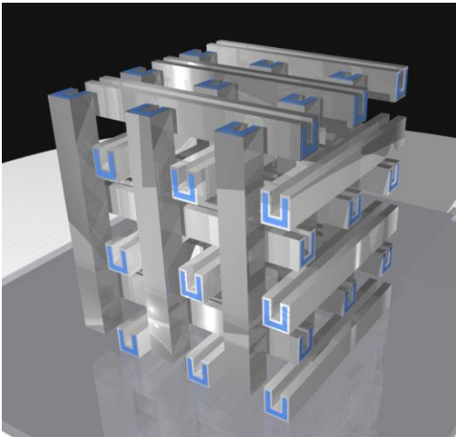
Fig.1: Artist’s view of a 3D photonic metamaterial composed of elongated split-ring resonators made by DLW of a polymeric backbone (blue) and subsequent coating via metal CVD.
