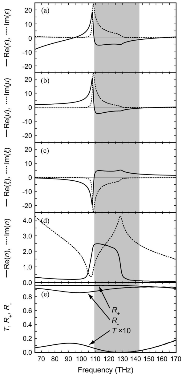
Fig. 7. (a)–(d) Retrieved effective parameters from numerical calculation of the complex transmittance and reflectances of the structure shown in Fig. 5 (a). (e) Calculated normal-incidence intensity transmittance ( T ) and reflectances ( R_+ , R_- ) of this structure.
